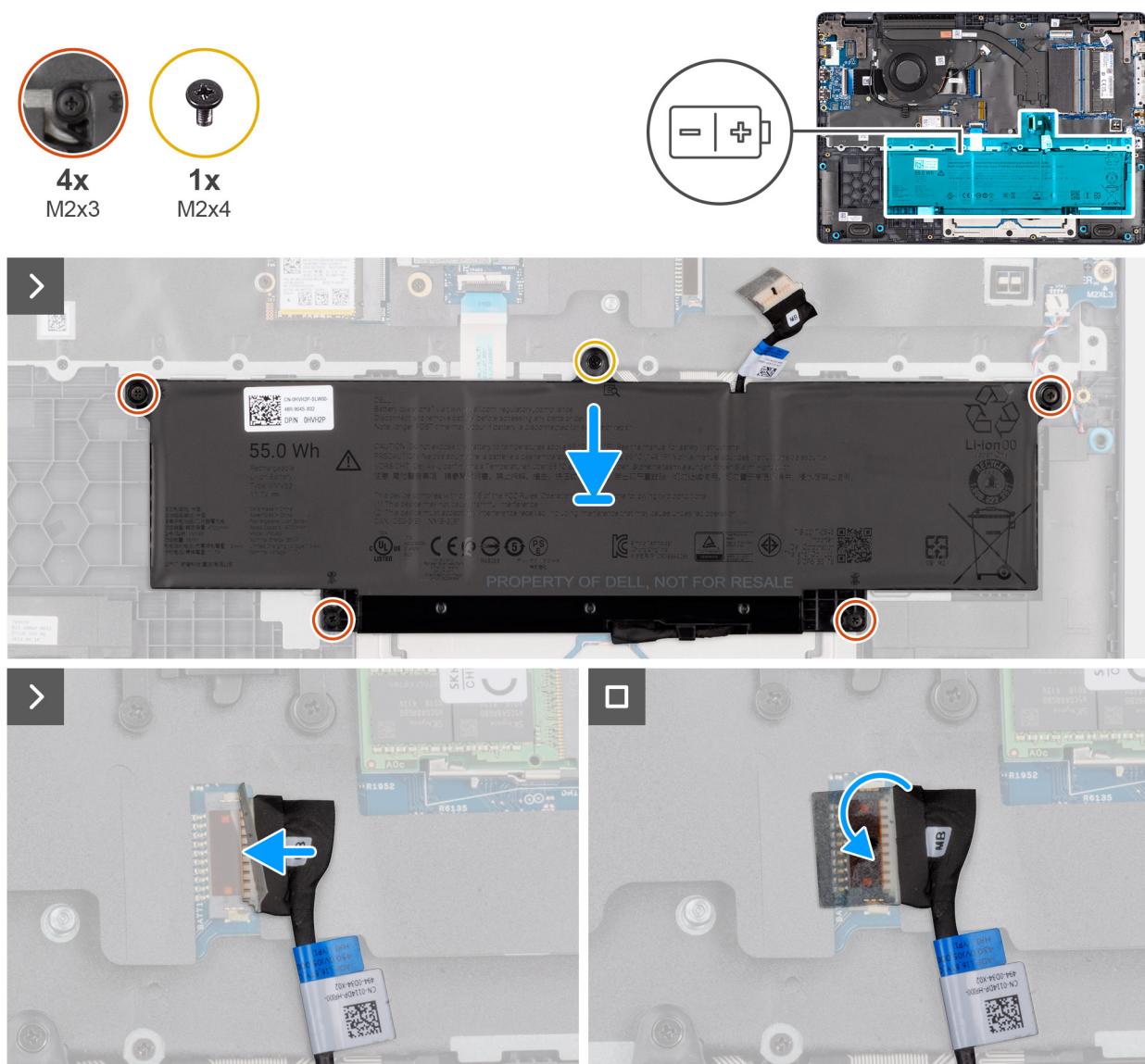
Obrazek 18. Installing the battery
