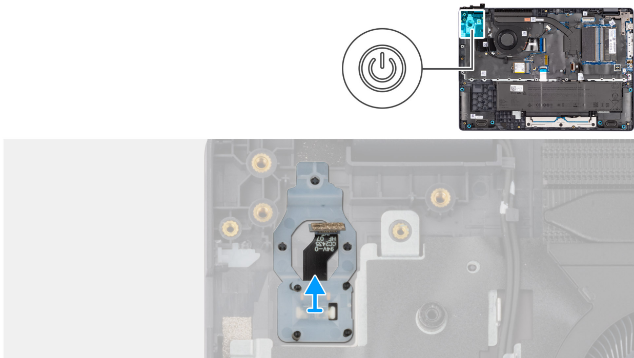
Obrázek 40. Removing the power button with fingerprint reader
