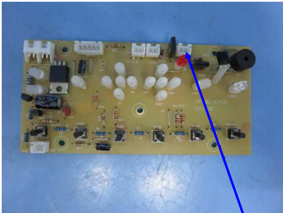
Control PCB view (the connector for water level indicator is optional)
