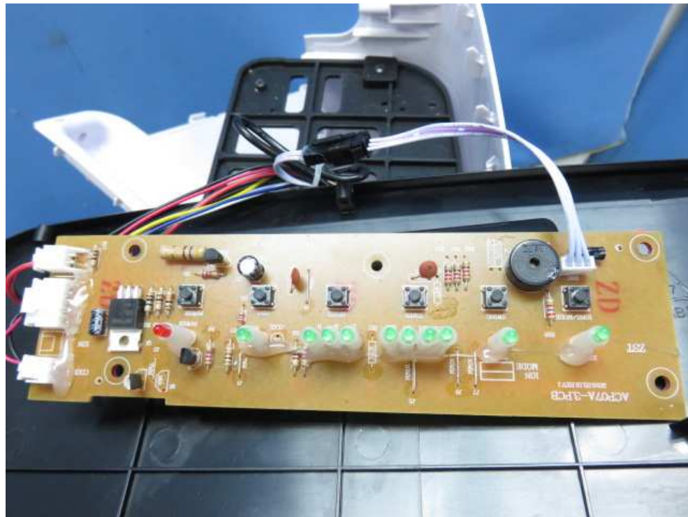
Control PCB board
