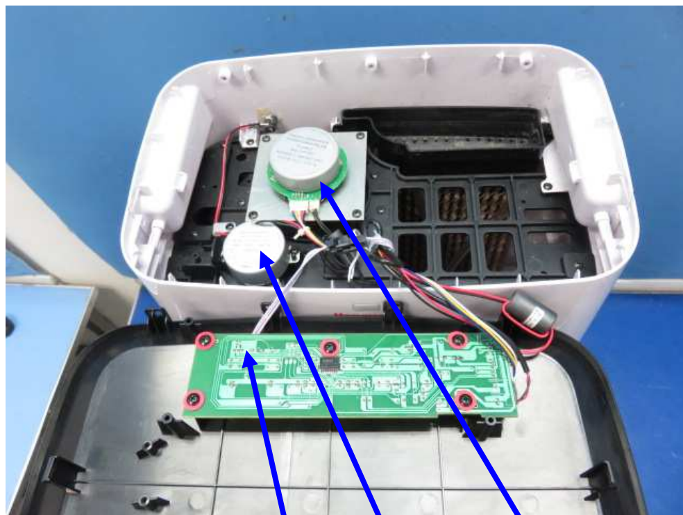
Inner view with top cover removed (location of control PCB board, sync. Motor and fan motor)
