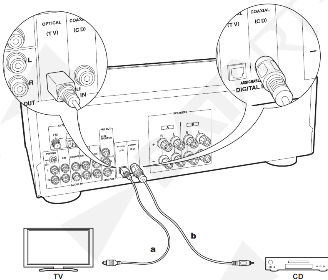
a: Kabel DIGITAL OPTICAL b: Kabel DIGITAL COAXIAL
