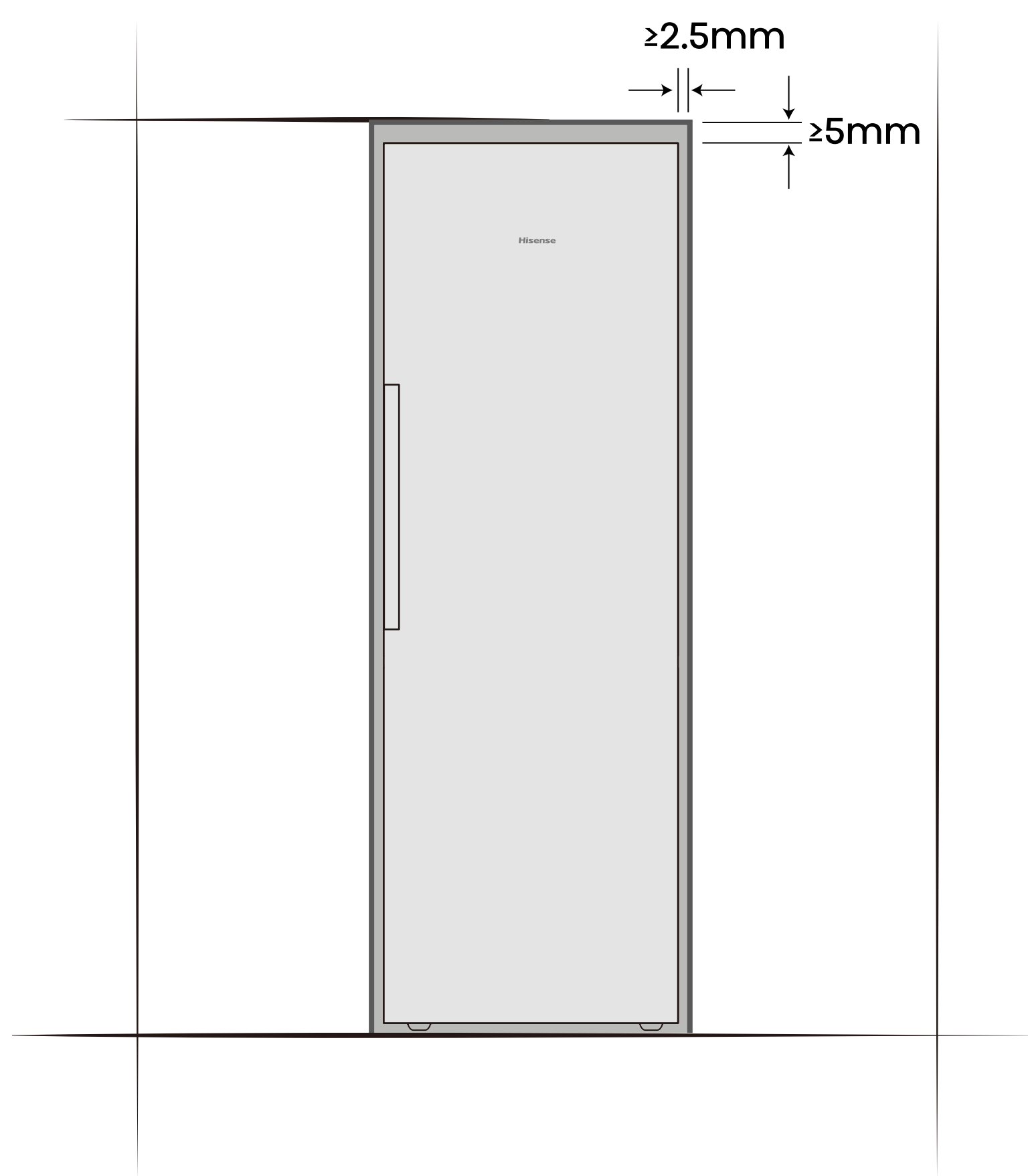
Front View
