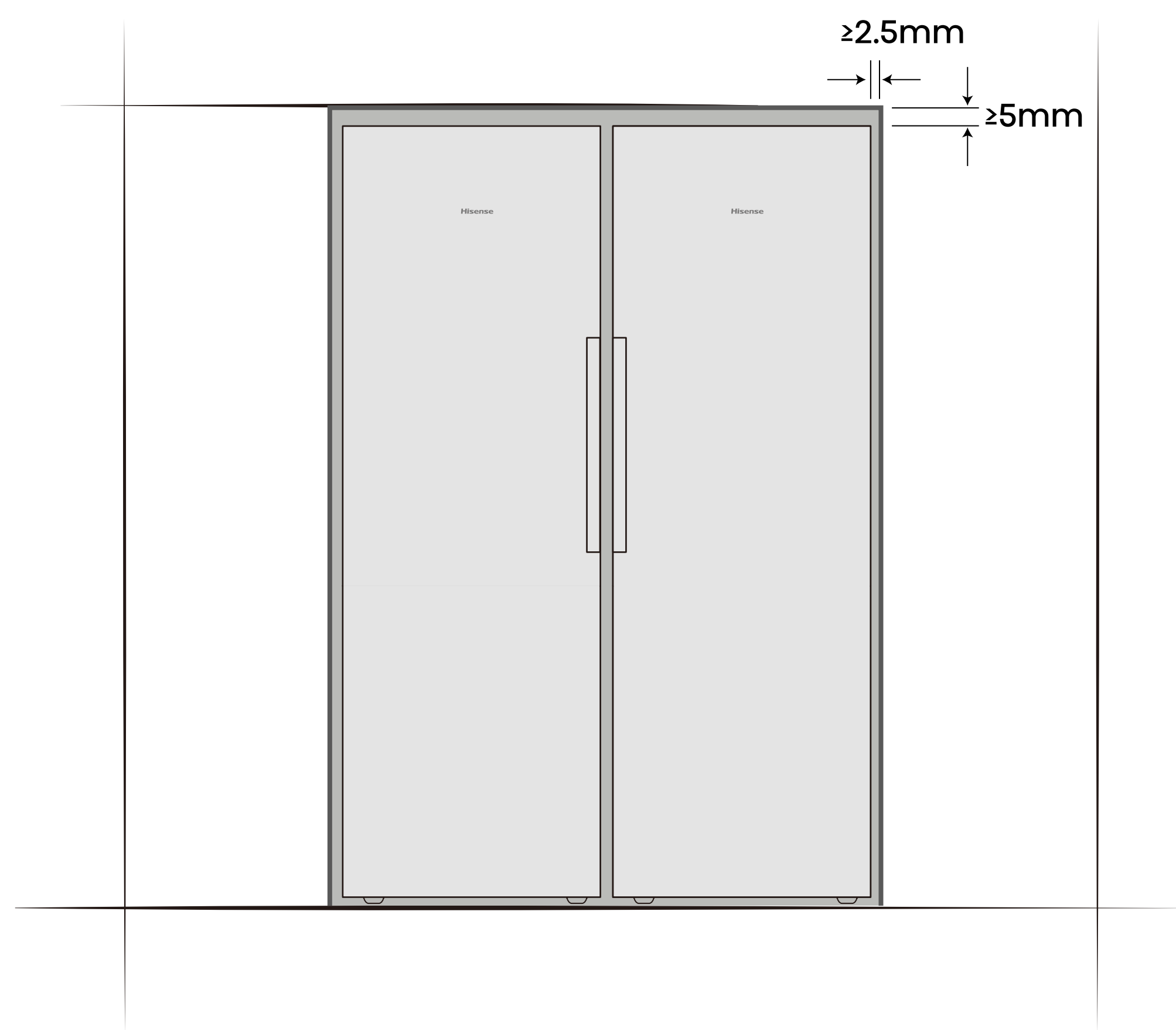
Front View
