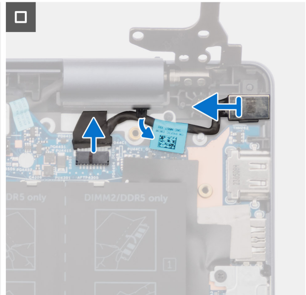
Figure 38. Removing the power-adapter port (for computers shipped with an aluminum chassis)
